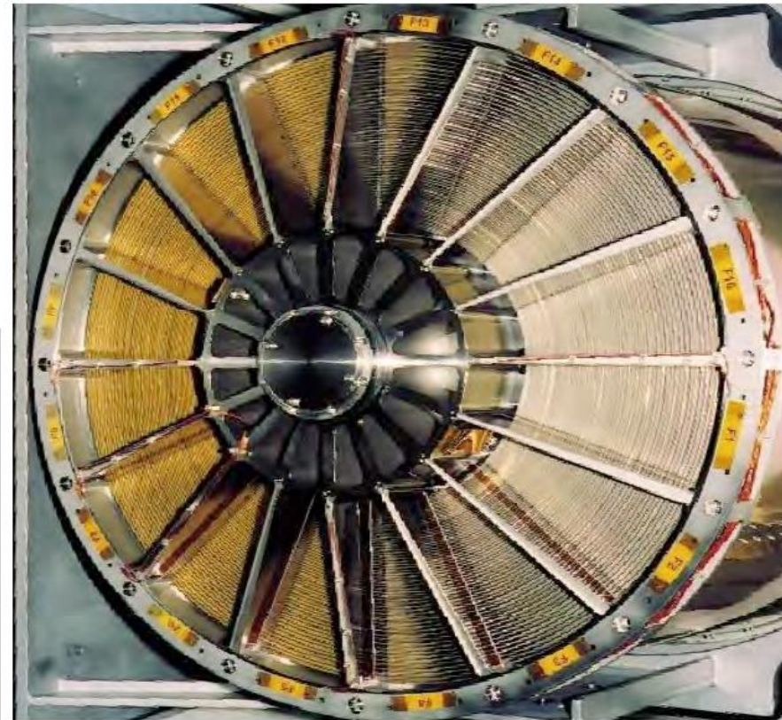
XMM-Newton mirrors during integration
