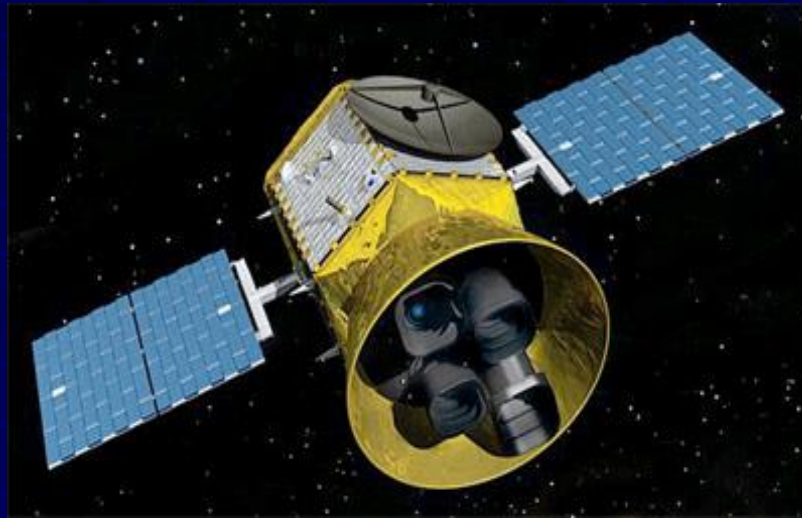
TESS
