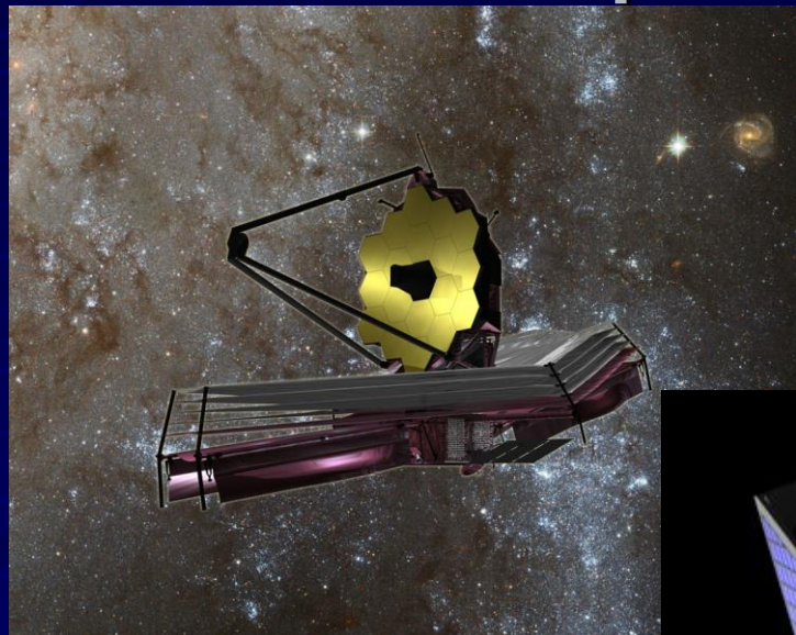
JWST (2022?)
