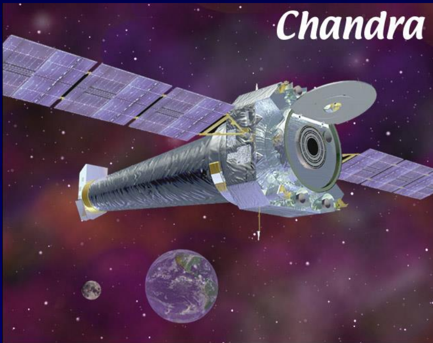
Chandra
