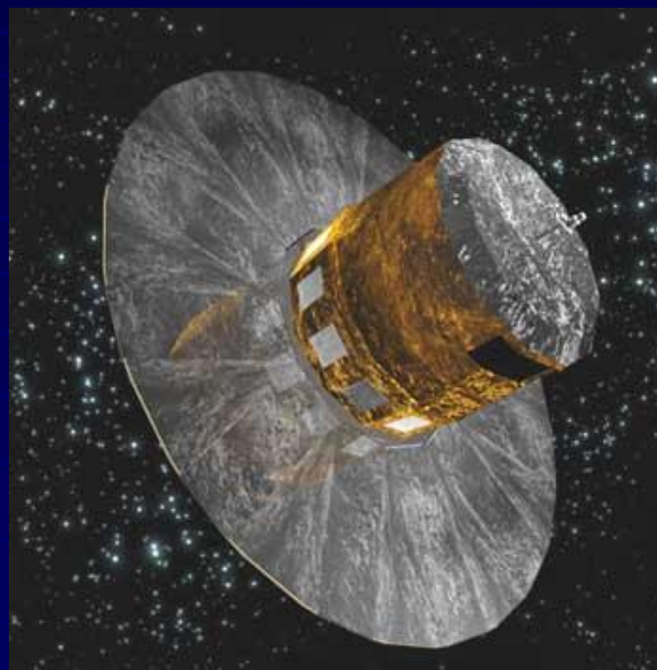
GAIA
