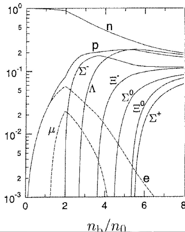
Relativistic mean-field model TM1 of Sugahara & Toki (1971)
