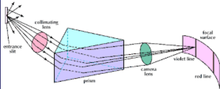
Principles of a Prism Spectrograph
