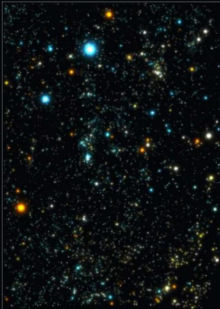
THE ROSAT X-RAY SKY AROUND ORION
