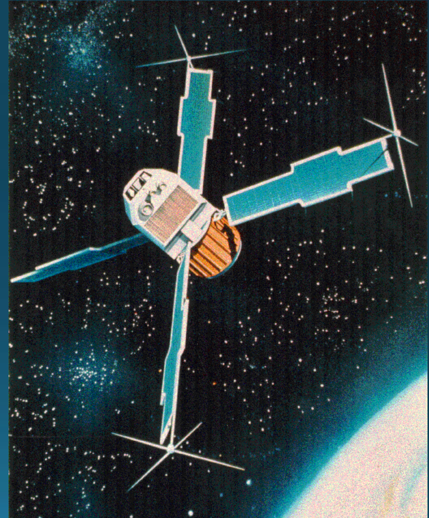
UHURU (1970)
